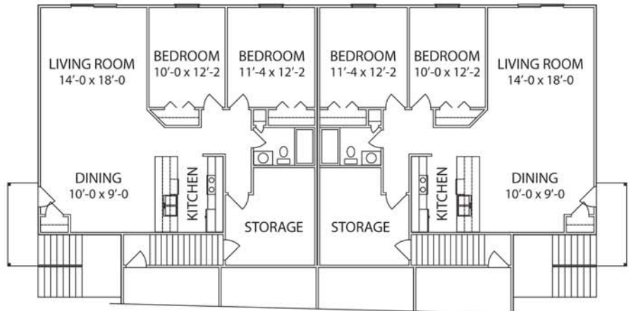
UPPER FLOOR
